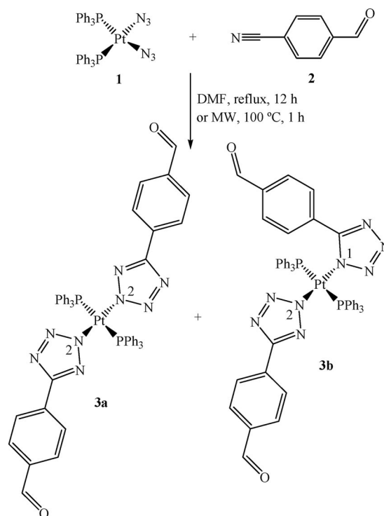
Scheme 1. N 2 N 2 -Bonded isomer 3a is the major product.
