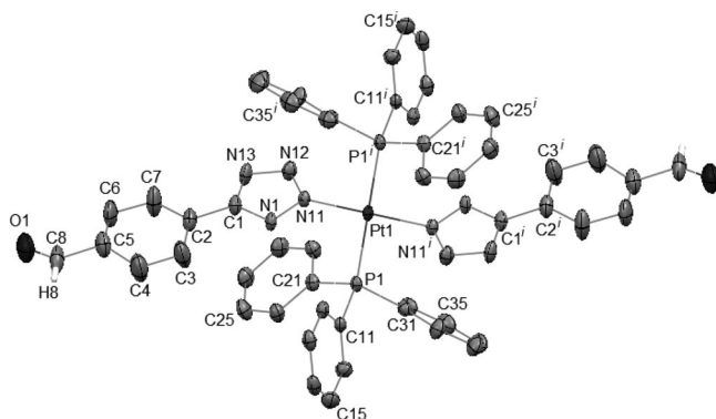
Figure 1. Molecular structure of 3a with atomic numbering scheme. Thermal ellipsoids are drawn at 30% probability. Symmetry operation to generate equivalent atoms: 1 -x , 2 -y , -z . Selected bond lengths [Å] and angles [°]: Pt1–N11 2.003(3), Pt1–P1 2.3336(11); P1–Pt1–N11 91.47(11), P1–Pt1–N11' 88.53(11).
