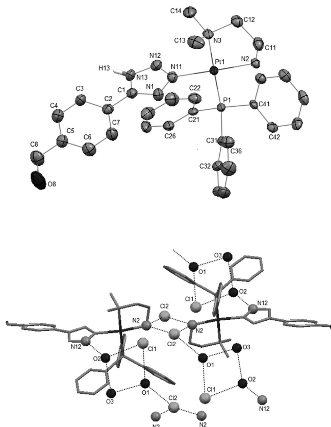
Figure 2. Molecular structure of 9 ·3H 2 O (top) with atomic numbering scheme (ellipsoids are drawn at 30% probability) and hydrogen-bonding interactions (bottom). Selected bond lengths [Å] and angles [°]: Pt1–P1 2.2558(15), Pt1–N2 2.036(5), Pt1–N3 2.141(5), Pt1–N11 2.005(6), N2–C11 1.486(8), N3–C12 1.509(9), N2–Pt1–N11 173.2(2), P1–Pt1–N3 177.16(17), P1–Pt1–N2 95.44(15), N2–Pt1–N3 83.6(2), N3–Pt1–N11 91.8(2). Intermolecular hydrogen bonds (dotted lines), D–H···A [ d (D···A), Å; \angle (DHA), °]: O1–H1A···O3 [2.774(10), 140.00], O1–H1B···Cl2 [2.880(9), 154.00], O2–H2A···N12 i [3.029(10), 178.00], O2–H2B···Cl1 [3.180(7), 162.00], N2–H2C···Cl2 [3.142(7), 150.00], N2–H2D···Cl2 ii [3.032(7), 142.00], O3–H3A···N1 [3.092(8), 161.00], O3–H3B···O2 [2.836(9), 165.00]. Symmetry codes to generate equivalent atoms: i : –1 + x , y , z ; ii : 2 – x , 1 – y , – z .
