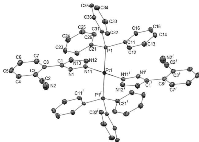
Figure 3. Thermal ellipsoid view of 12a with atomic numbering scheme. Thermal ellipsoids are drawn at 30% probability. Symmetry transformations used to generate the equivalent atoms i : -x , -y , -z . Selected bond lengths [Å] and angles [°]: Pt1–N11 2.018(3), Pt1–P1 2.3403(10), N11–Pt1–N11' 180.0, N11–Pt1–P1' 92.30(9), N11–Pt1–P1 87.70(9), P1–Pt1–P1' 180.0.
